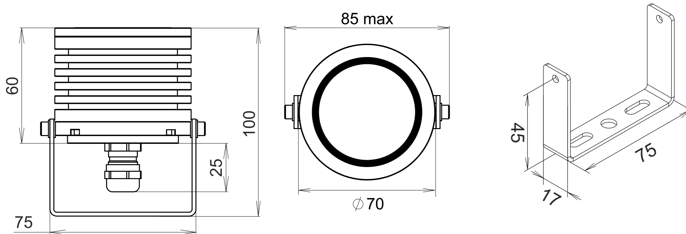
IntiSPOT color dynamic surface-mounted luminaire dimensional drawing
