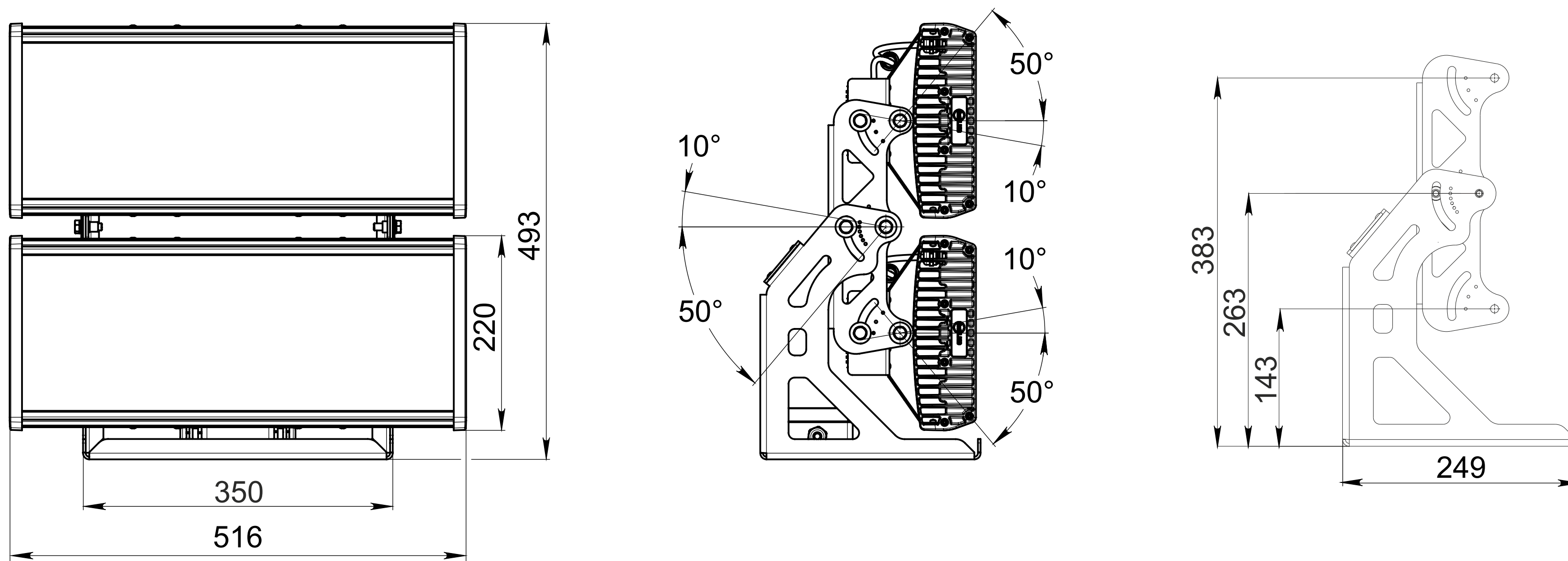
IntiSTARK big-block white color luminaire dimensional drawing
