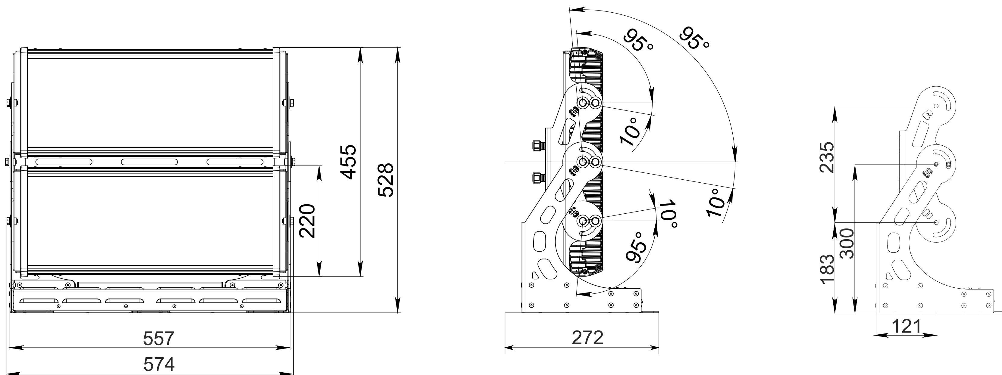
IntiSTARK big-block color dynamic luminaire dimensional drawing
