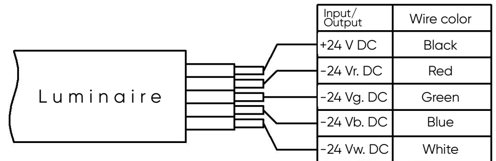
LACE RGBW luminaire connections diagram
