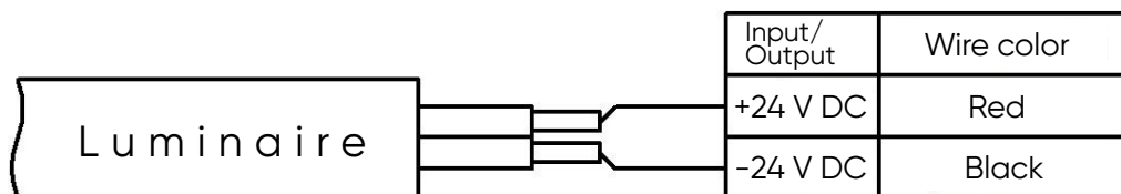
LACE white color luminaire connections diagram
